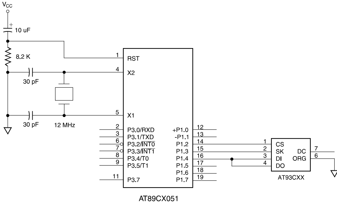
Figure 1. 3-Wire Configuration
