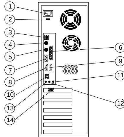
Slim Desktop (SDT)
