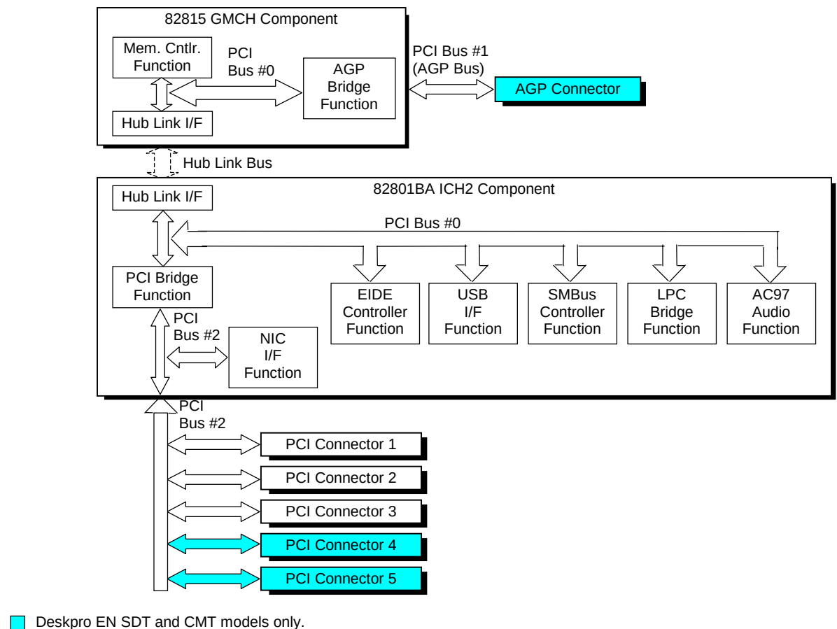
Figure 4-1. PCI Bus Devices and Functions
