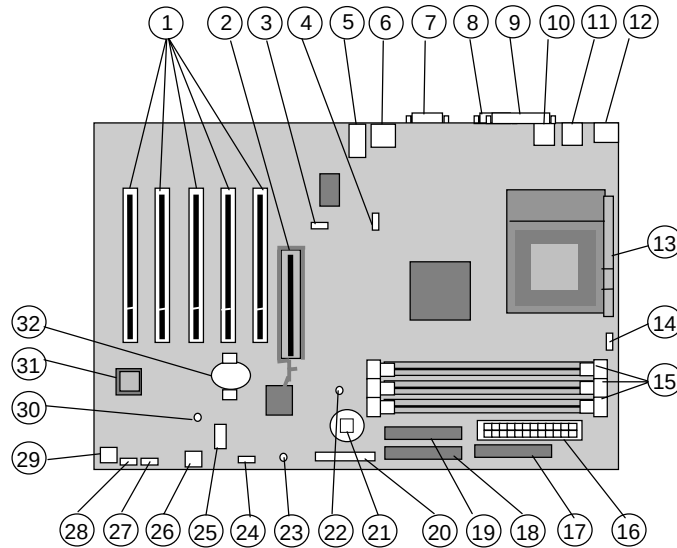
System Board PCA# 010630 or 011032
