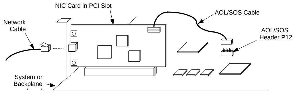
Figure 5-16. Remote System Alert Implementation (Generic Representation)
