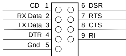
Figure 5-4. COM1 Serial Interface Header (Deskpro EN SFF system board only)
