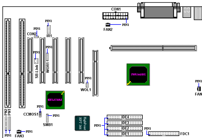
Figure 2-5. All Connectors and Headers for the BE6
