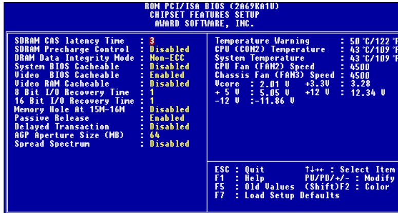
Fig 3-5 Chipset Features Setup
