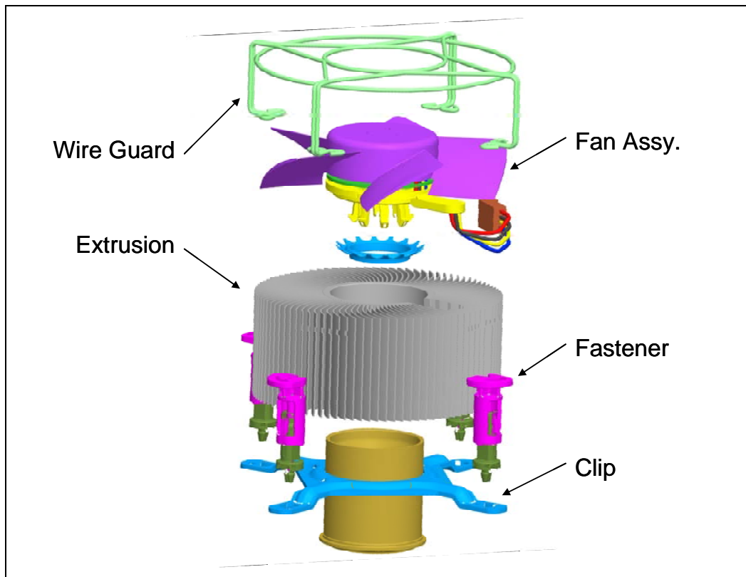
Figure 19. Intel® RCFH-4 Reference Design – Exploded View
