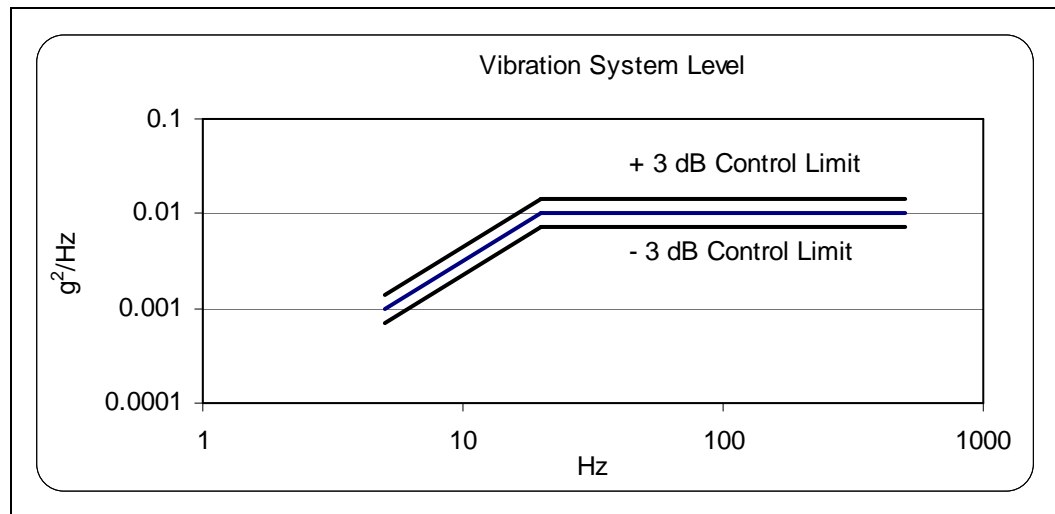
Figure 11. Random Vibration PSD
