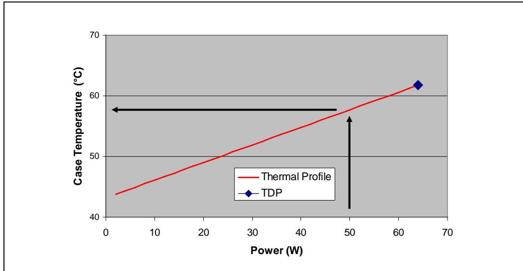
Figure 3. Example Thermal Profile
