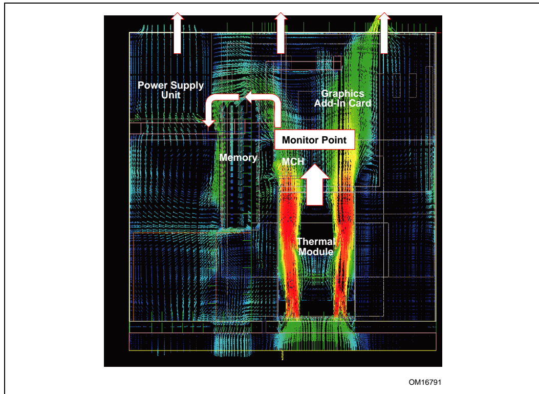
Figure 68. System Airflow Illustration with System Monitor Point Area Identified
