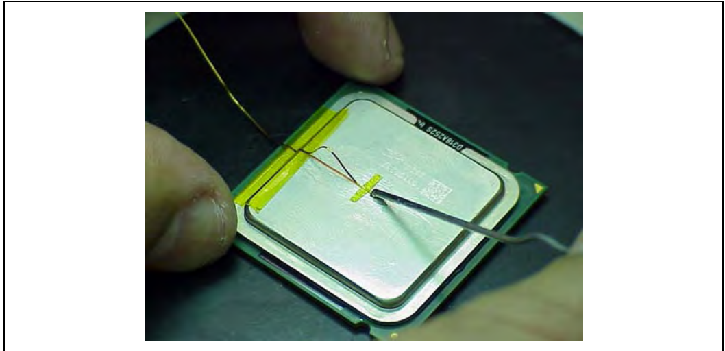
Figure 47. Applying Flux to the Thermocouple Bead
