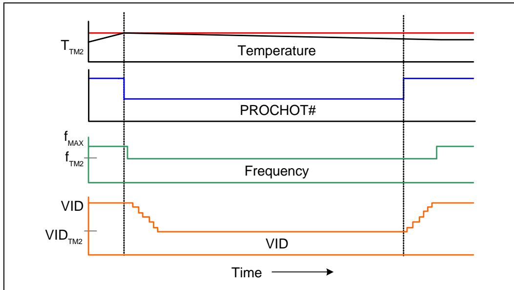
Figure 8. Thermal Monitor 2 Frequency and Voltage Ordering
