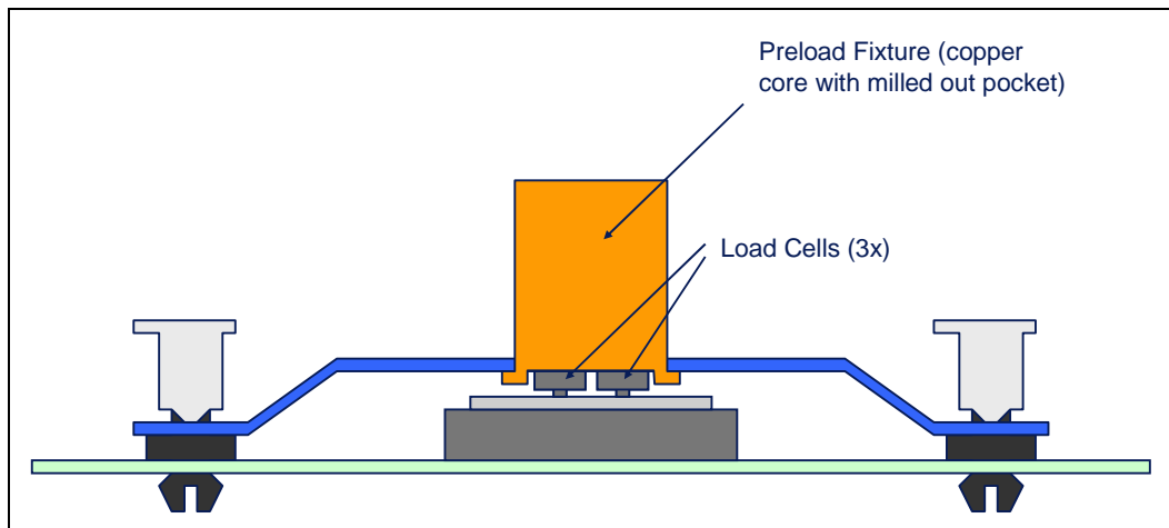
Figure 33. Preload Test Configuration
