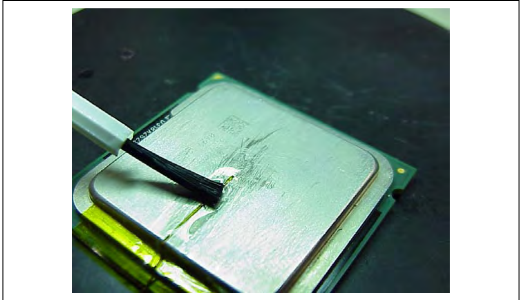
Figure 58. Removing Excess Adhesive from IHS
