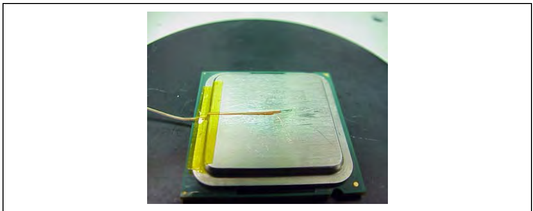
Figure 41. Securing Thermocouple Wires with Kapton* Tape Prior to Attach
