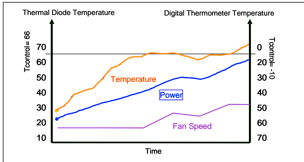
Figure 9. T_{CONTROL} for Digital Thermal Sensor
