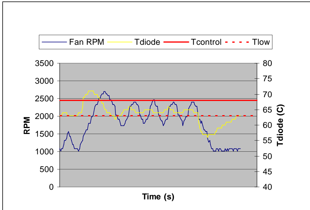
Figure 64. Temperature Range = 5 °C
