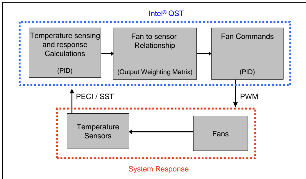
Figure 24. Intel® QST Overview
