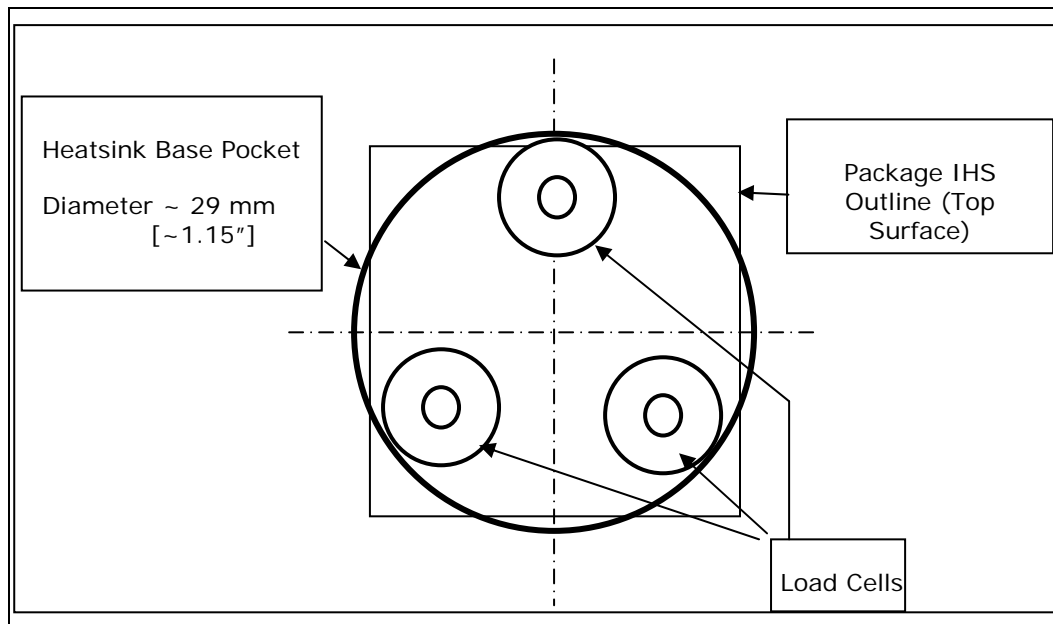
Figure 31. Load Cell Installation in Machined Heatsink Base Pocket – Bottom View
