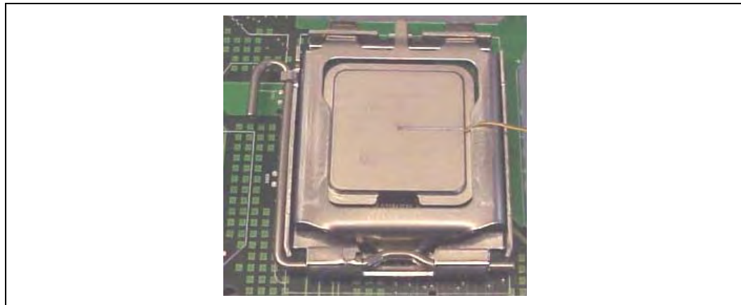
Figure 38. IHS Groove per Figure 35 Orientation Relative to the LGA775 Socket
