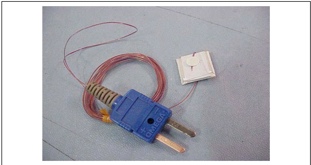
Figure 34. Omega Thermocouple
