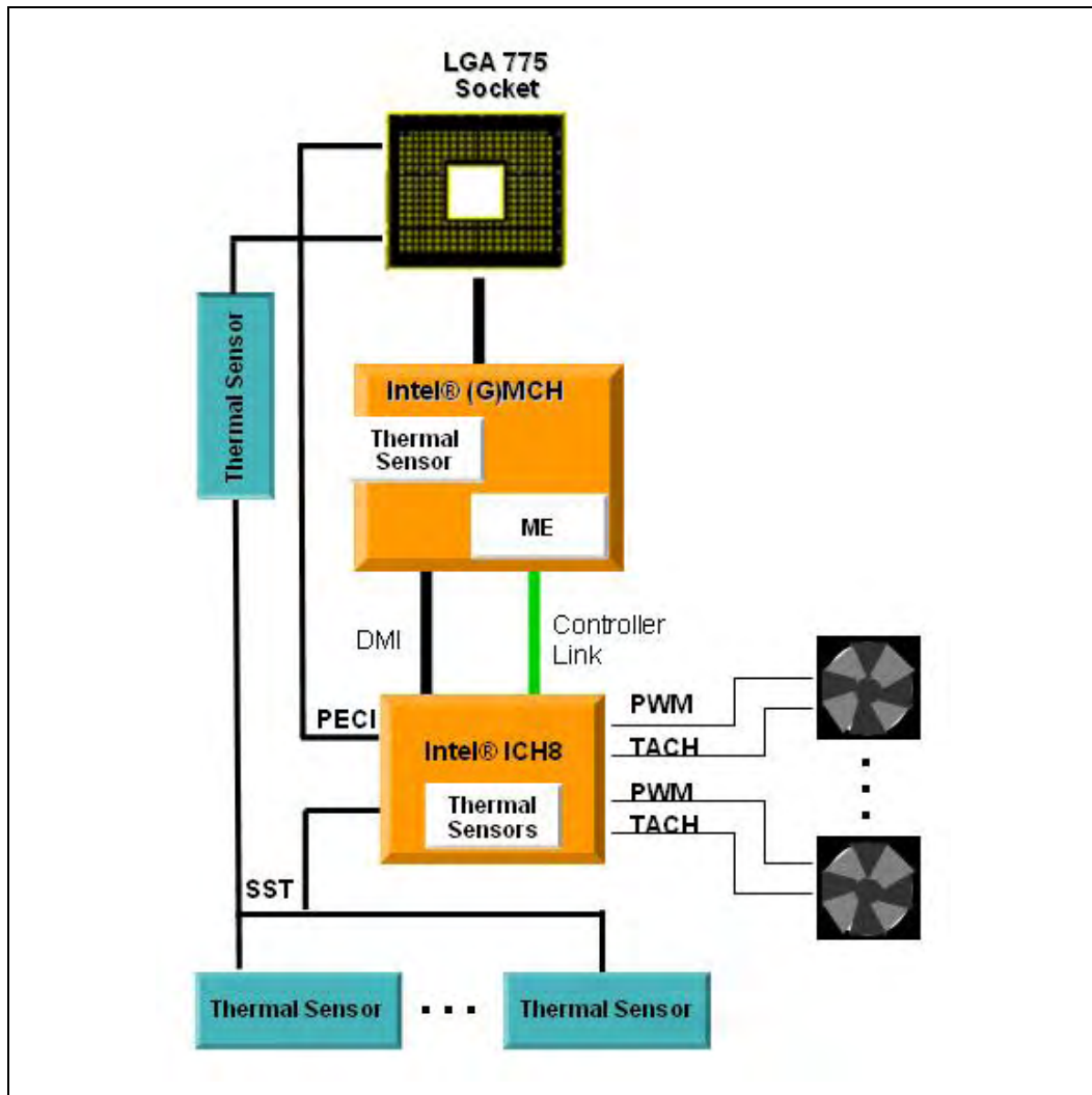
Figure 27. Example Acoustic Fan Speed Control Implementation
