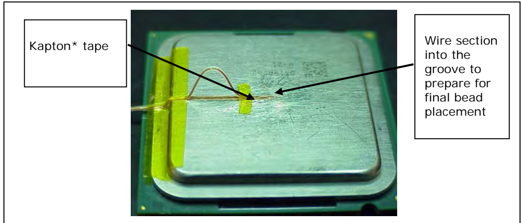
Figure 44. Detailed Thermocouple Bead Placement
