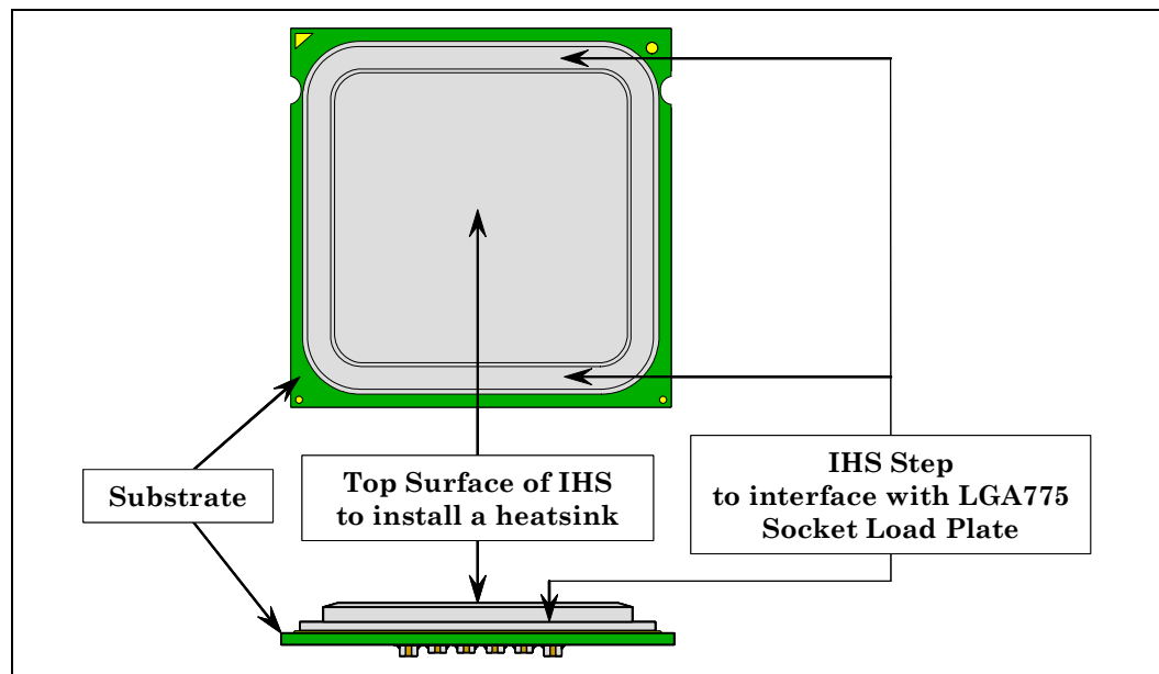
Figure 1. Package IHS Load Areas
