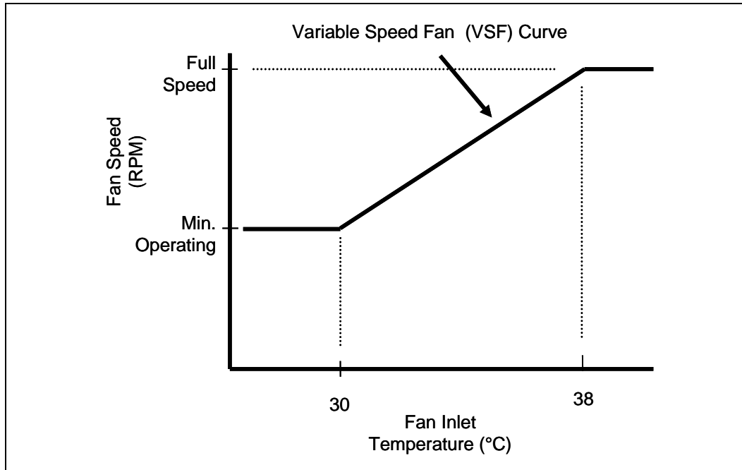
Figure 61. Thermistor Set Points
