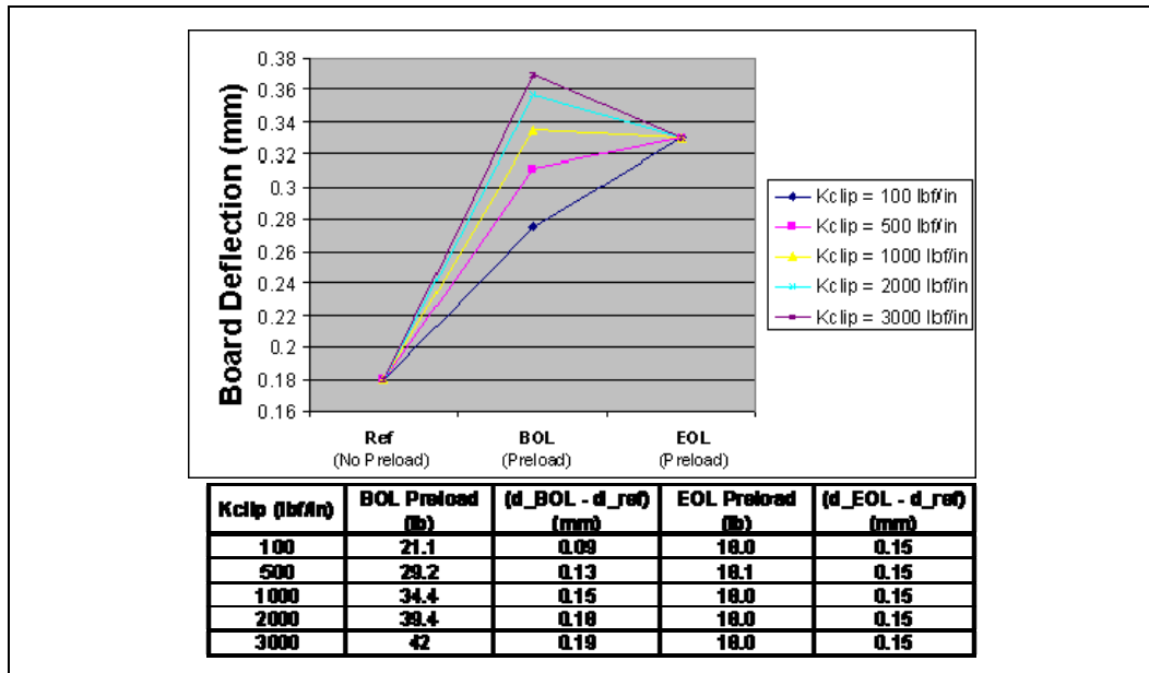
Figure 30. Example: Defining Heatsink Preload Meeting Board Deflection Limit
