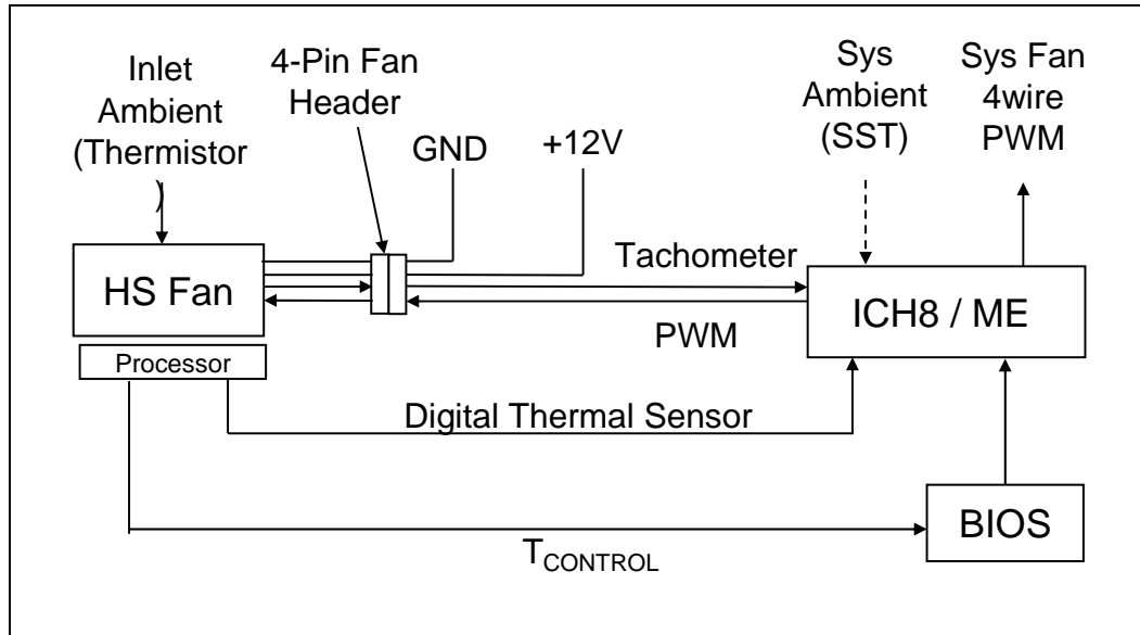
Figure 62. Example Fan Speed Control Implementation
