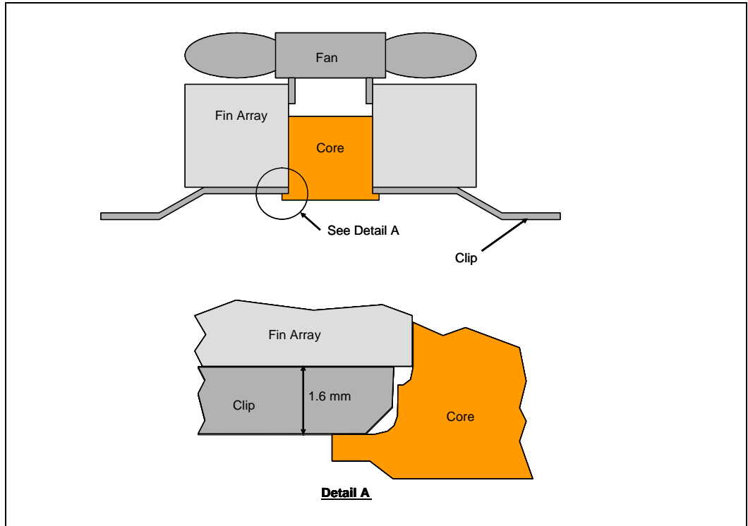
Figure 23. Critical Core Dimension
