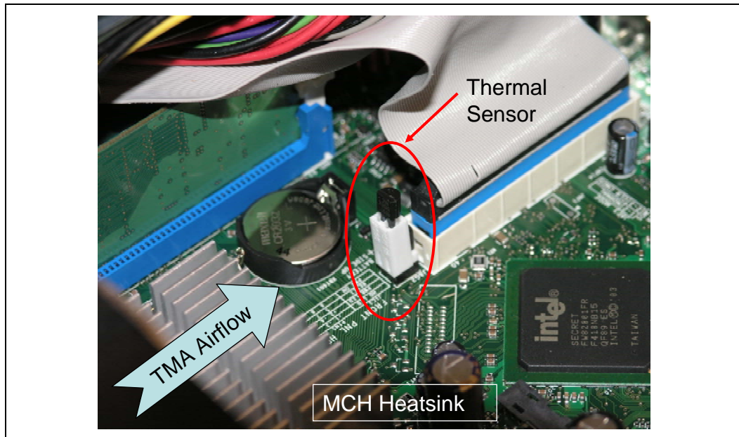
Figure 69. Thermal sensor Location Illustration
