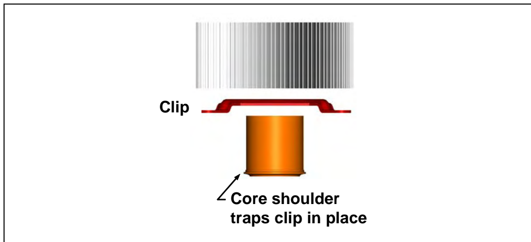
Figure 21. Reference Clip/Heatsink Assembly
