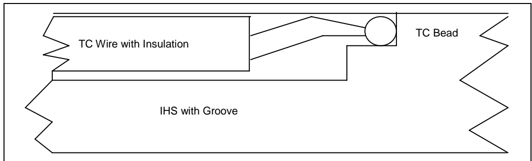
Figure 44. Detailed Thermocouple Bead Placement
