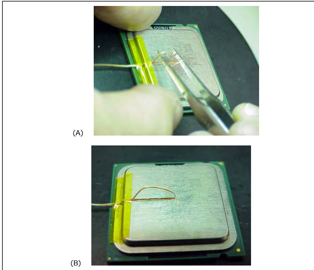
Figure 42. Thermocouple Bead Placement
