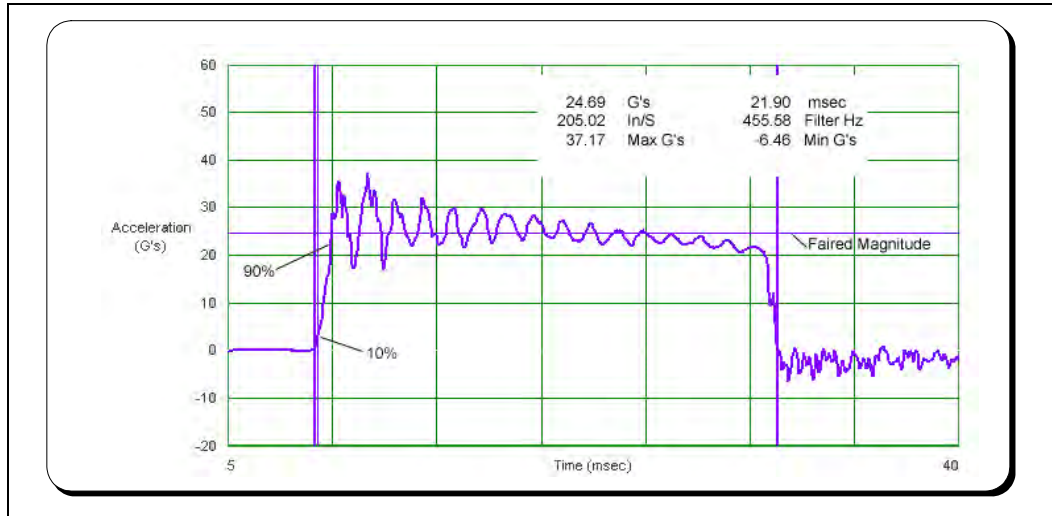
Figure 12. Shock Acceleration Curve
