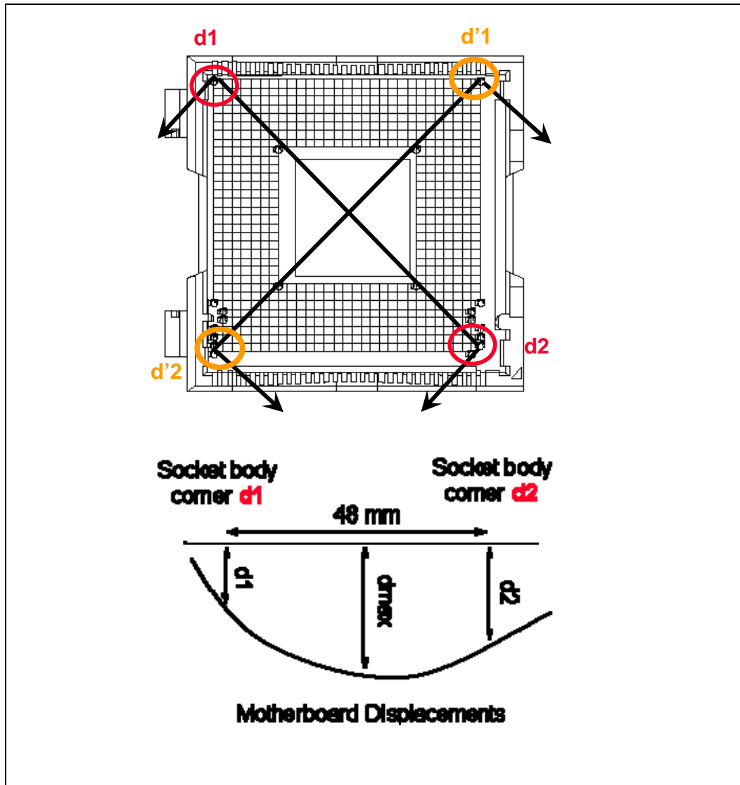
Figure 29. Board Deflection Definition
