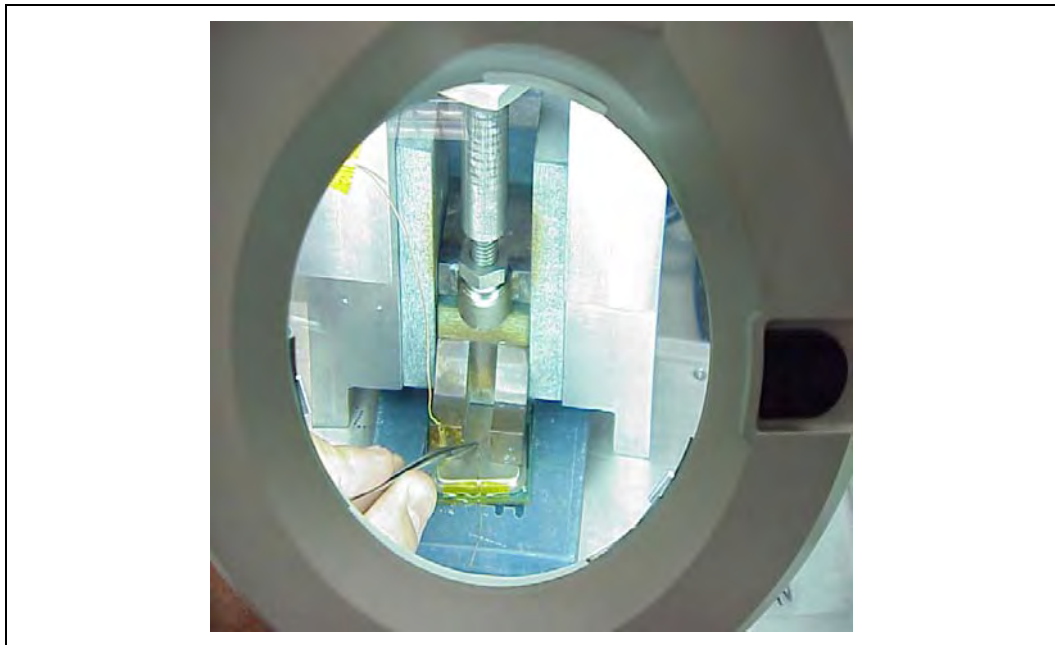
Figure 52. Moving Solder back onto Thermocouple Bead
