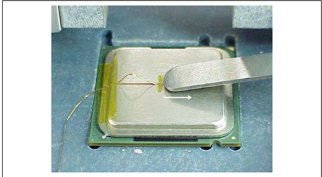
Figure 53. Removing Excess Solder
