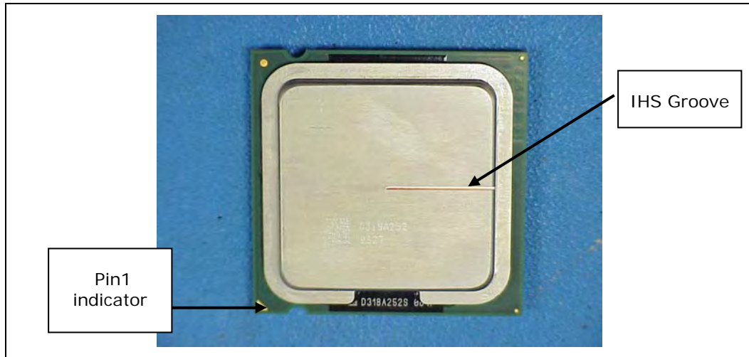
Figure 37. IHS Groove per Figure 35 on the 775-LAND LGA Package
