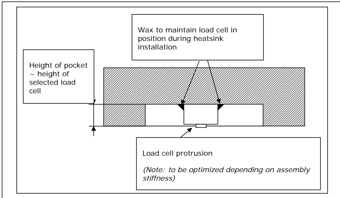
Figure 32. Load Cell Installation in Machined Heatsink Base Pocket – Side View
