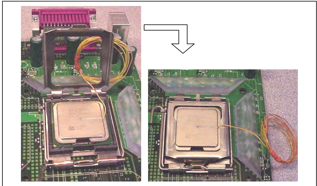
Figure 60. Thermocouple Wire Management
