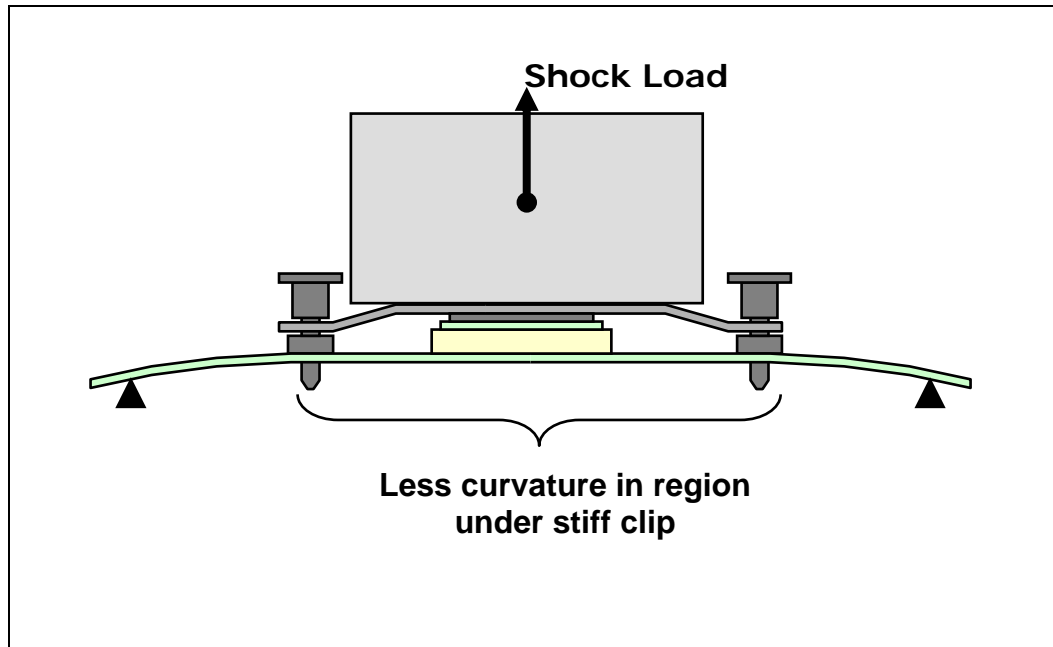
Figure 20. Upward Board Deflection During Shock
