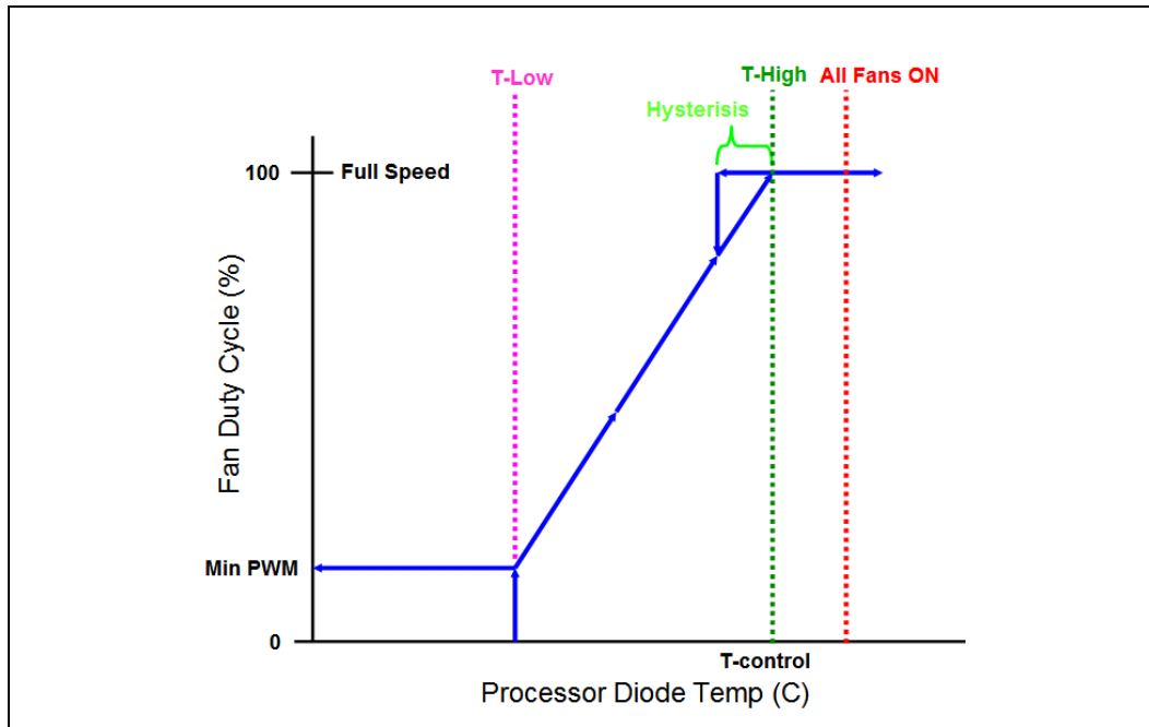
Figure 67. FSC Definition Example
