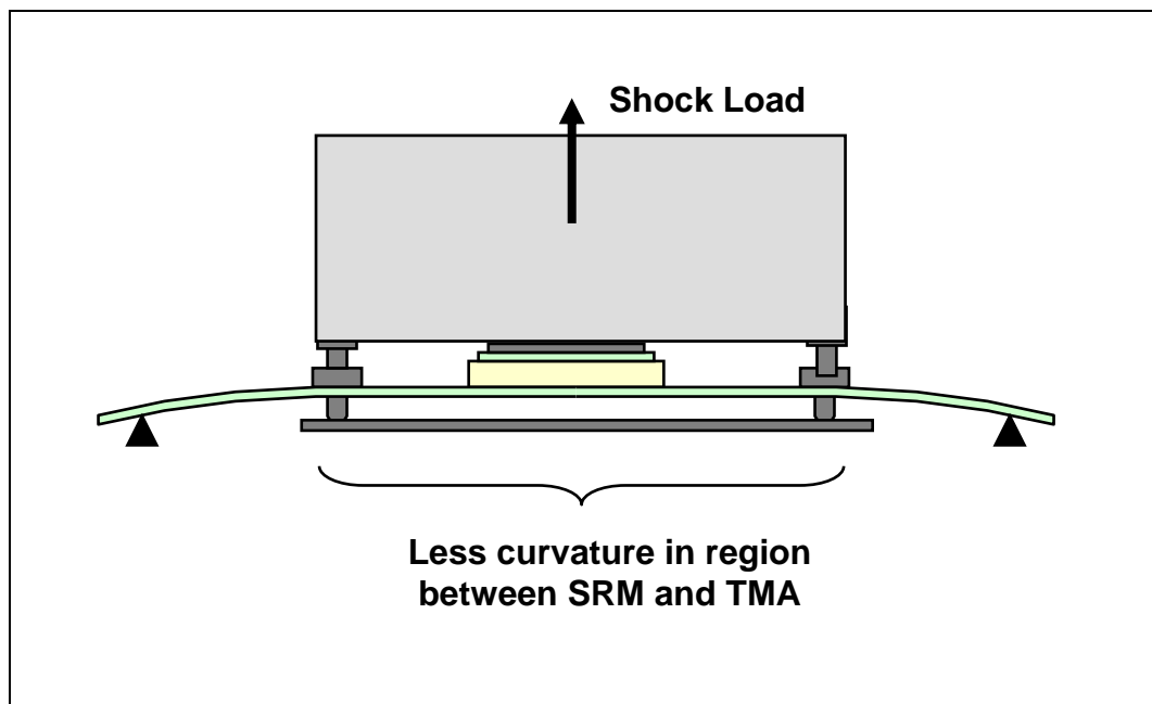
Figure 14. Upward Board Deflection During Shock
