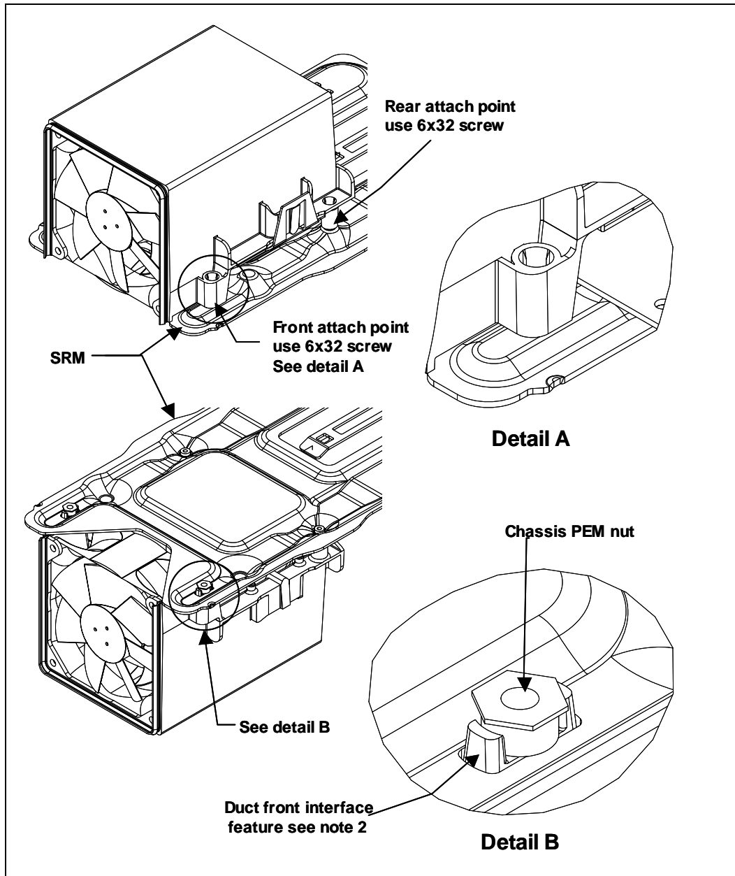
Figure 16. Thermal Module Attach Pointes and Duct-to-SRM Interface Features
