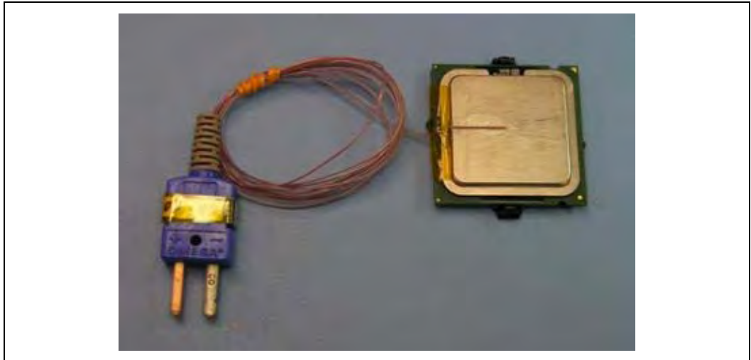
Figure 59. Finished Thermocouple Installation
