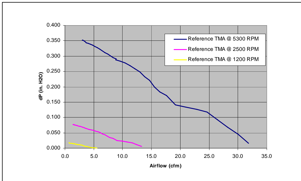
Figure 10. Effective TMA Fan Curves with Reference Extrusion
