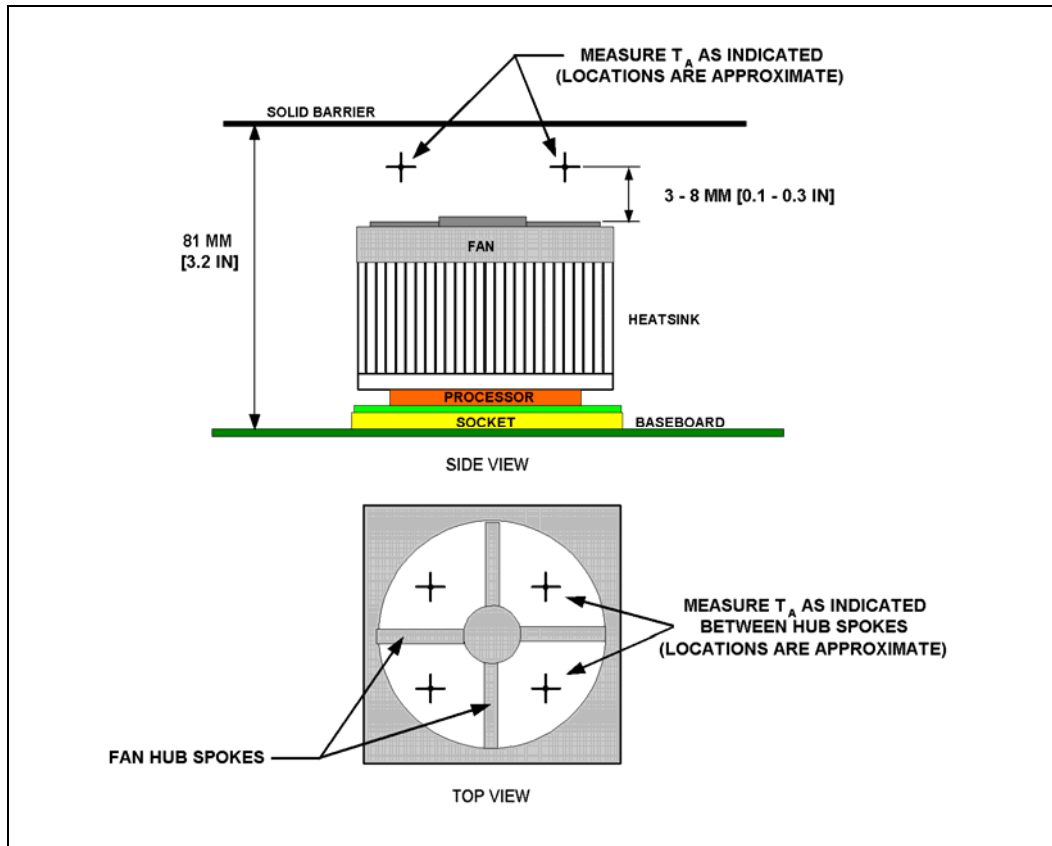
Figure 5. Locations for Measuring Local Ambient Temperature, Active ATX Heatsink
