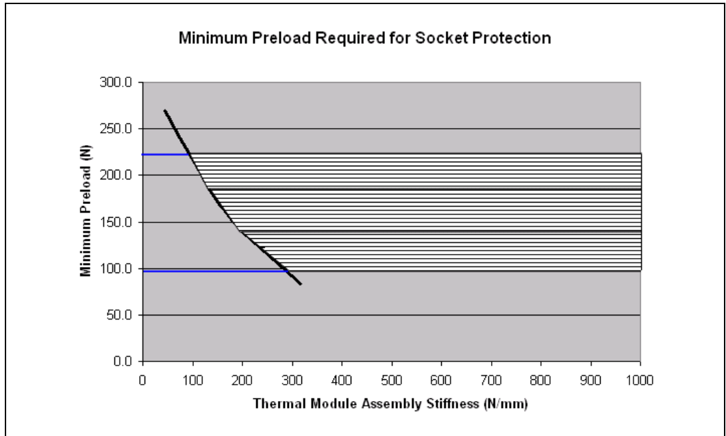
Figure 15. Minimum Required Processor Preload to Thermal Module Assembly Stiffness
