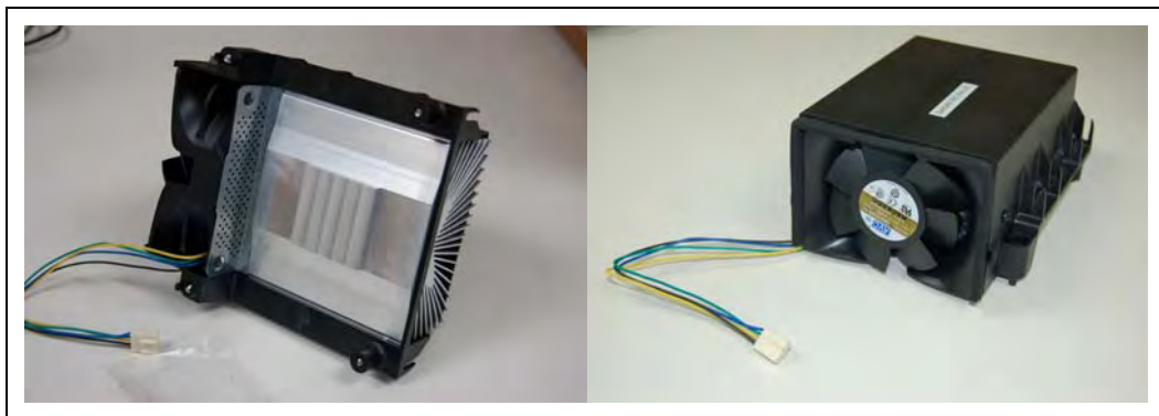
Figure 13. Intel Type II TMA 65W Reference Design
