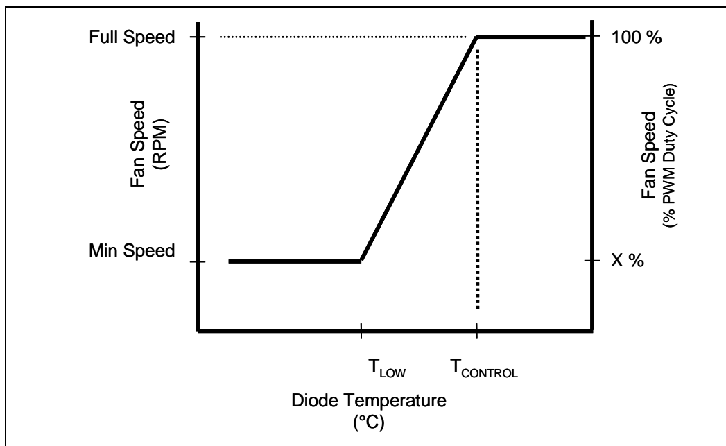
Figure 63. Fan Speed Control
