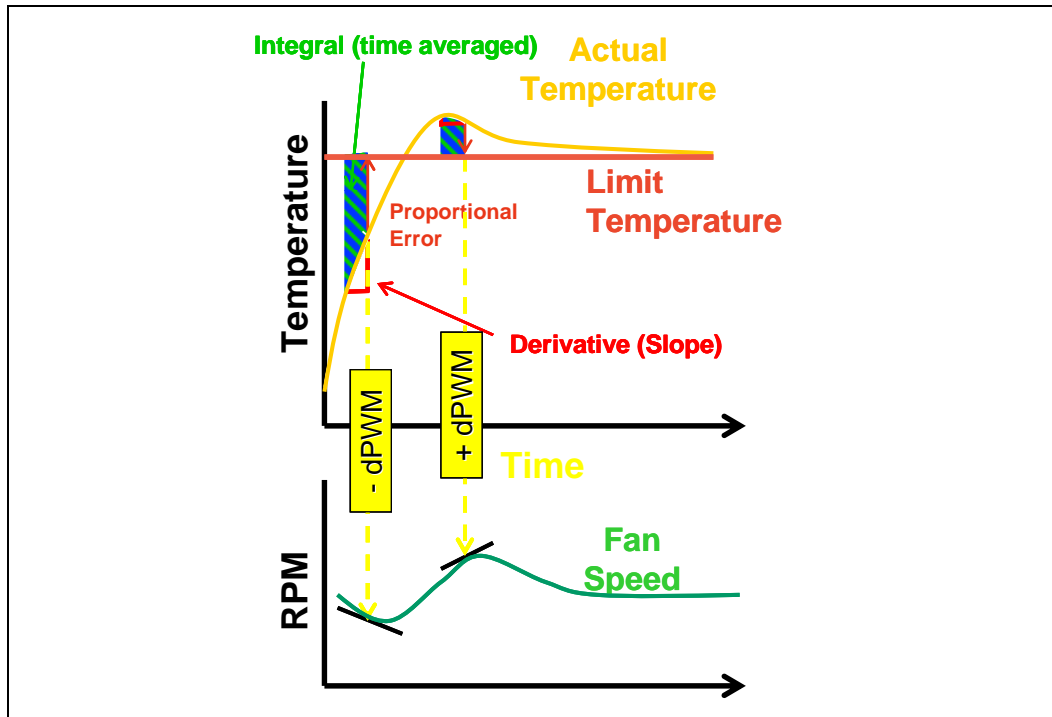
Figure 25. PID Controller Fundamentals
