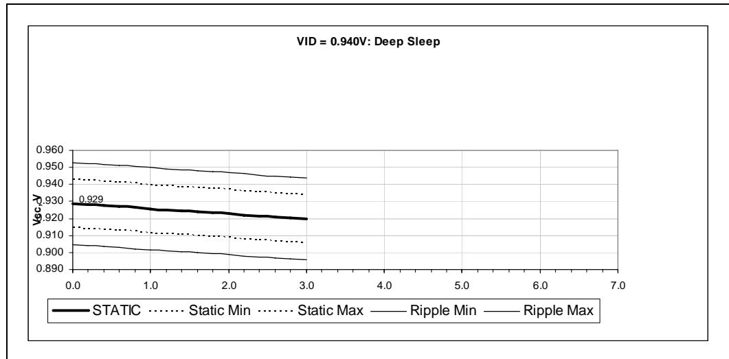
Figure 3-4. Illustration of Deep Sleep State V_{CC} Static and Ripple Tolerances for the Celeron M Processor ULV: VID=0.940 V
