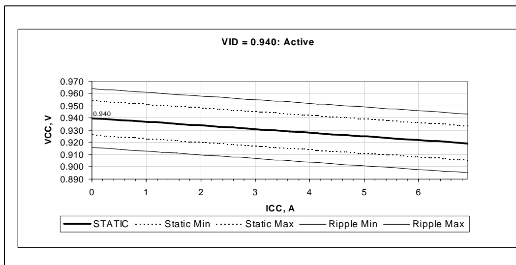
Figure 3-3. Illustration of Active State V_{CC} Static and Ripple Tolerances for the Celeron M Processor ULV: VID=0.940 V
