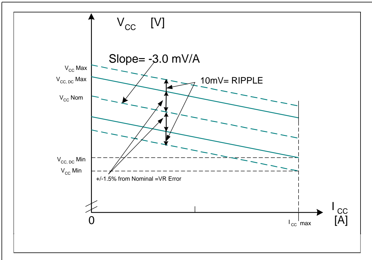
Figure 3-5. Active V_{CC} and I_{CC} Load Line for the Celeron M Processor: Standard Voltage and Ultra Low Voltage
