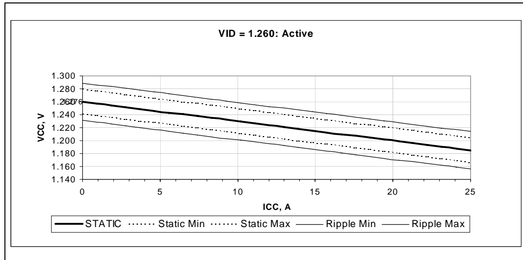
Figure 3-1. Illustration of Active State V_{CC} Static and Ripple Tolerances for the Celeron M Processor: VID=1.260 V
