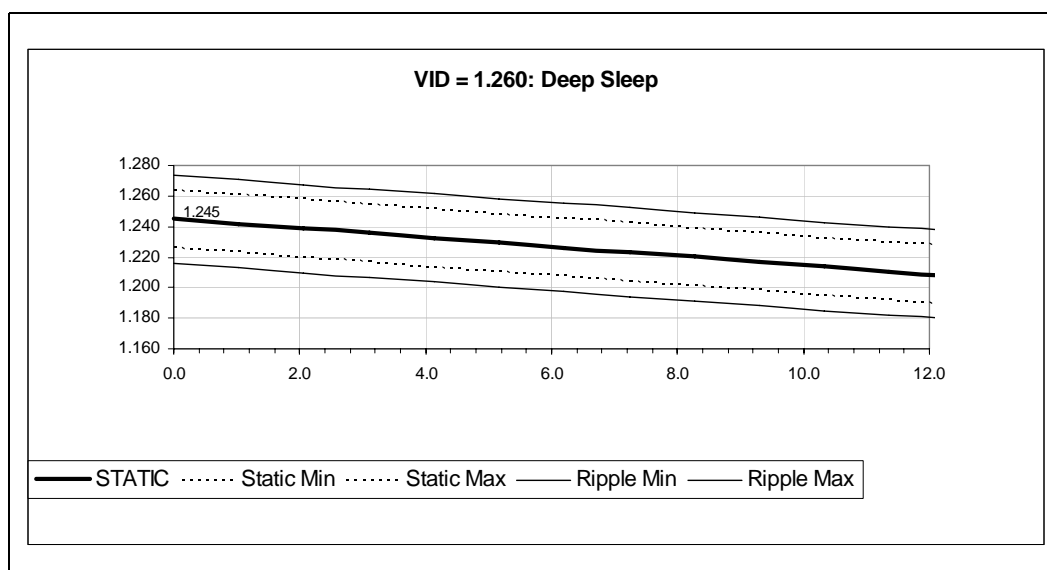
Figure 3-2. Illustration of Deep Sleep State V CC Static and Ripple Tolerances for the Celeron M Processor (Deep Sleep State): VID=1.260 V
