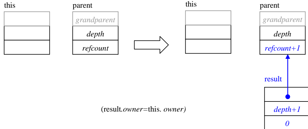
Figure 8: Effect of allocate_child_of(parent)
