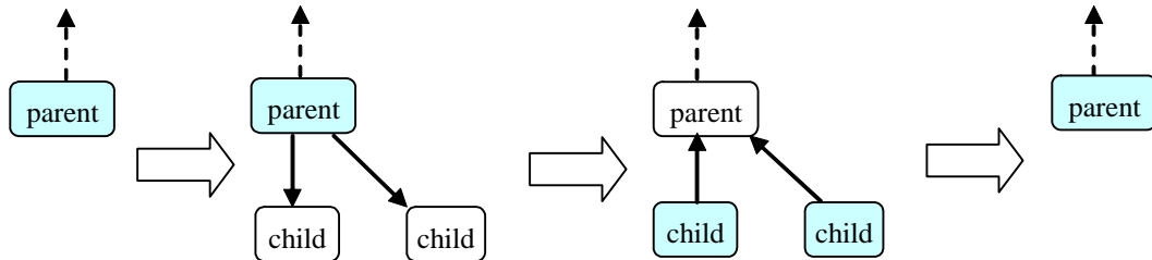
Figure 3: Blocking style
