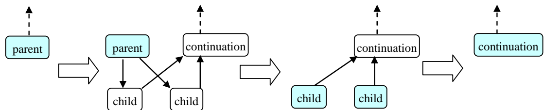
Figure 2: Continuation-passing style
