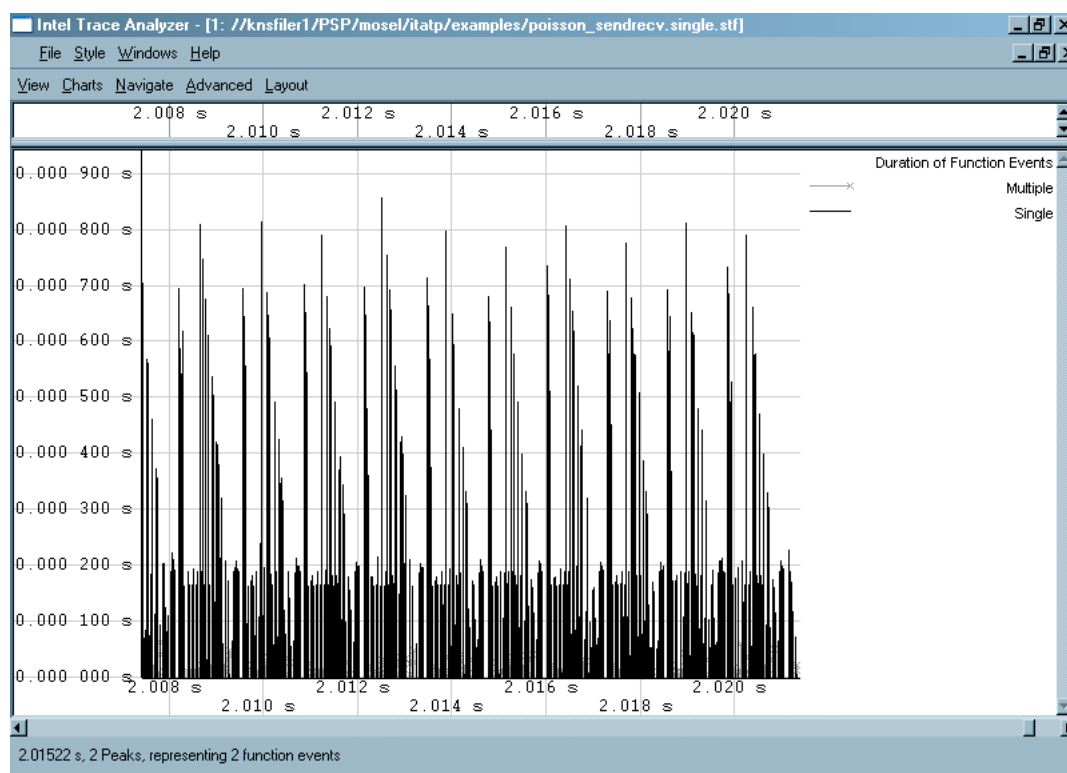
Figure 4.8. Qualitative Timeline
