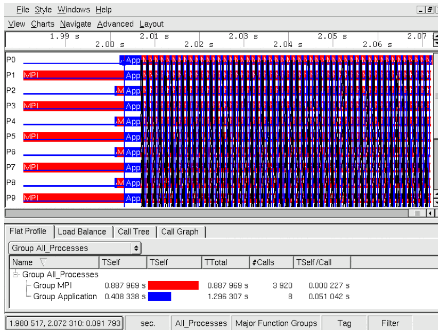
Figure 1.6. Zoomed result
