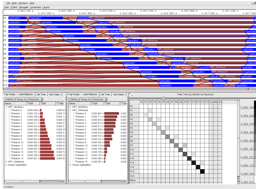
Figure 1.9. Many Charts
