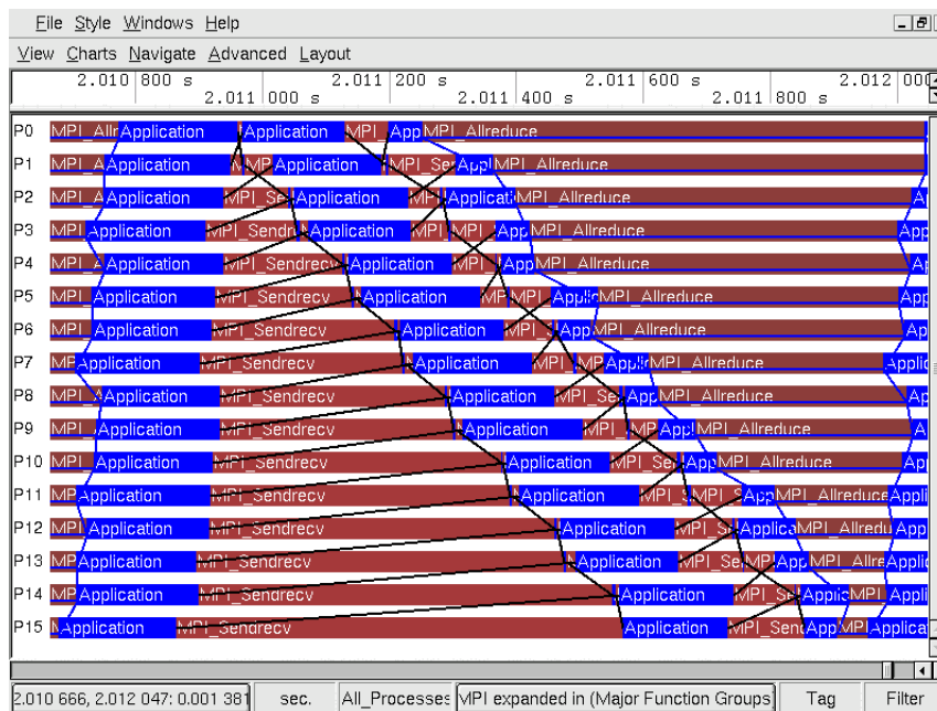
Figure 1.8. MPI ungrouped
