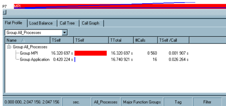
Figure 4.24. Function Profile
