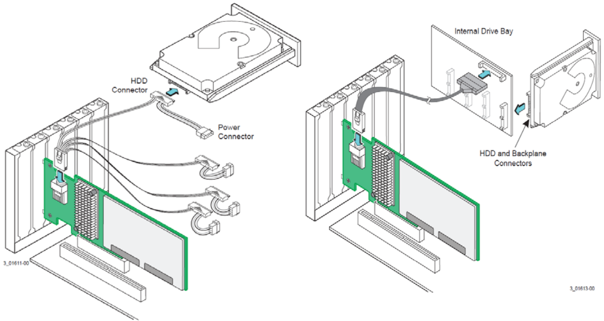
Figure 7. Internal SAS cables for Connecting SAS or SATA devices
