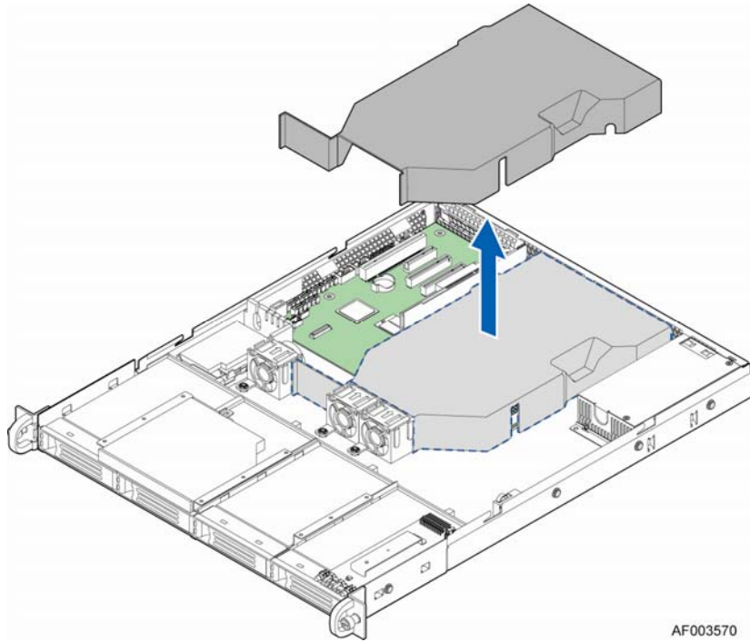
Figure 13. Intel® Server System R1304BTLSHBN Air Duct
