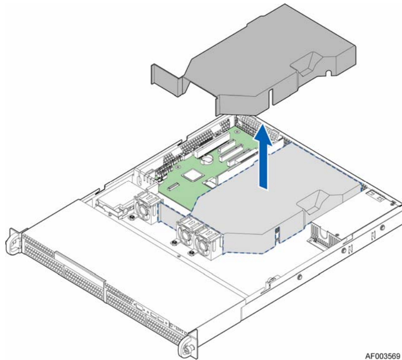
Figure 12. Intel® Server System R1304BTSSFAN/R1304BTLSFAN Air Duct
