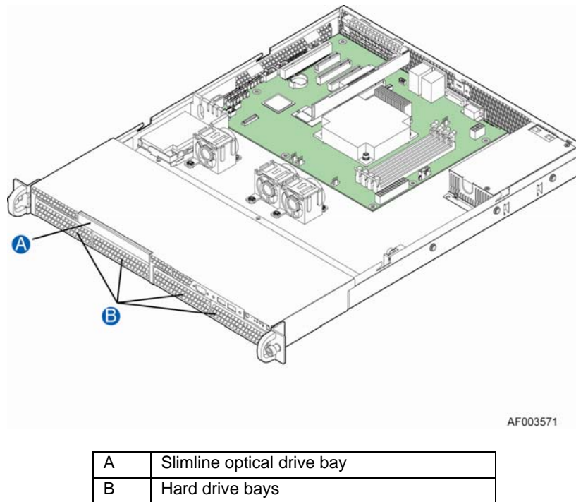
Figure 14. Intel® Server Systems R1304BTSSFAN/R1304BTLSFAN Drive Bays
