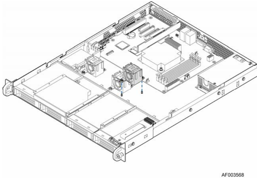
Figure 11. Intel® Server System R1304BTLSHBN Fan Module Assembly
