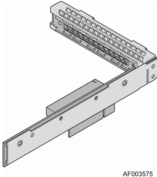
Figure 17. PCI-E Riser Card Assembly For Intel® Server System R1304BTSSFAN, R1304BTLSSFAN and R1304BTLSHBN
