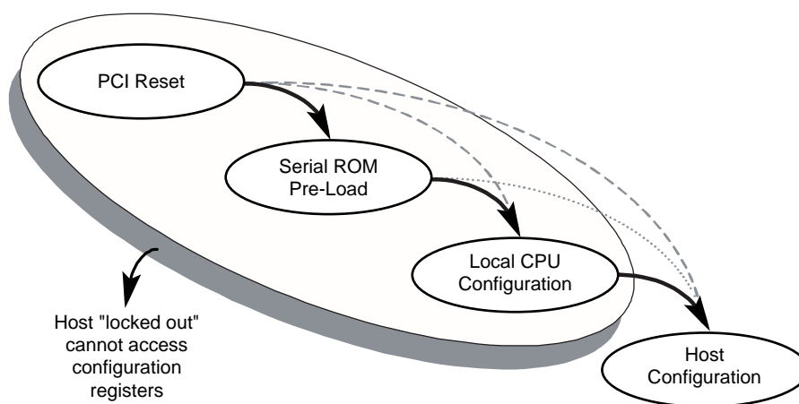
Figure 1. 21554 Initialization Sequence
