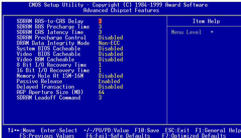
Figure 3-6. Menu de l'Advanced Chipset Features
