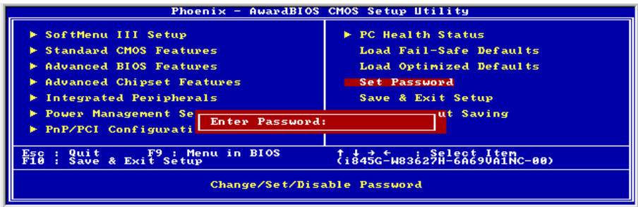
Abb. 3-14. Set Password
